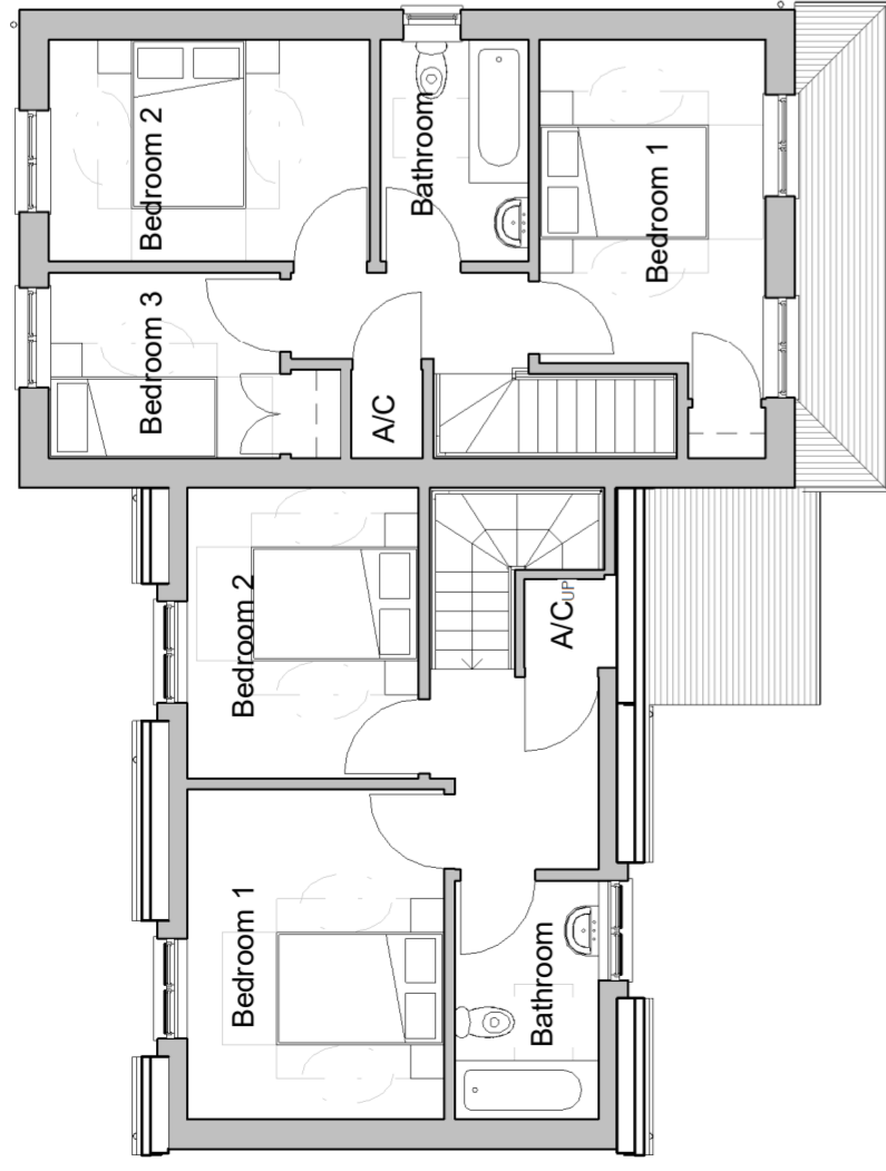
Houses 1 & 2 - First Floor Plan as Proposed 1 : 100
