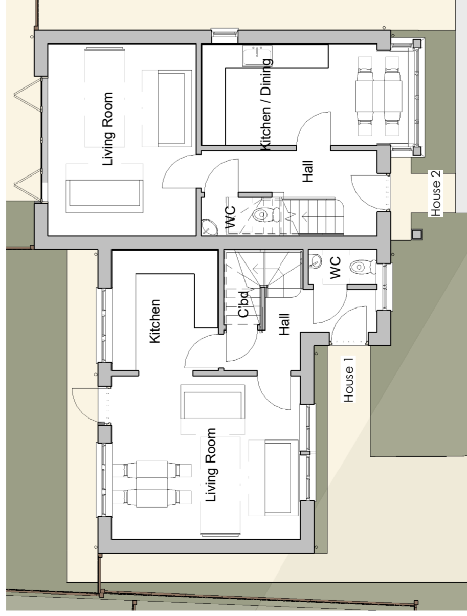
Houses 1 & 2 - Ground Floor Plan as Proposed 1 : 100
